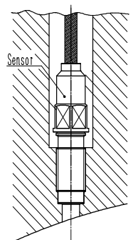
CAS-15S mounting example
